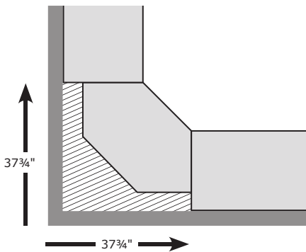
Corner section with two 22 \frac{7}{8} " deep frames.
