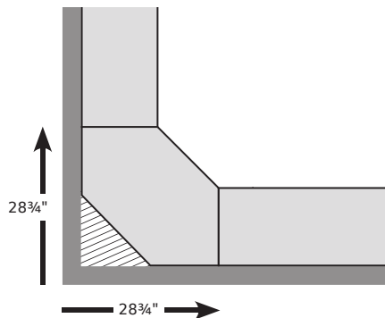
Corner section with two 13 \frac{3}{4} " deep frames.
